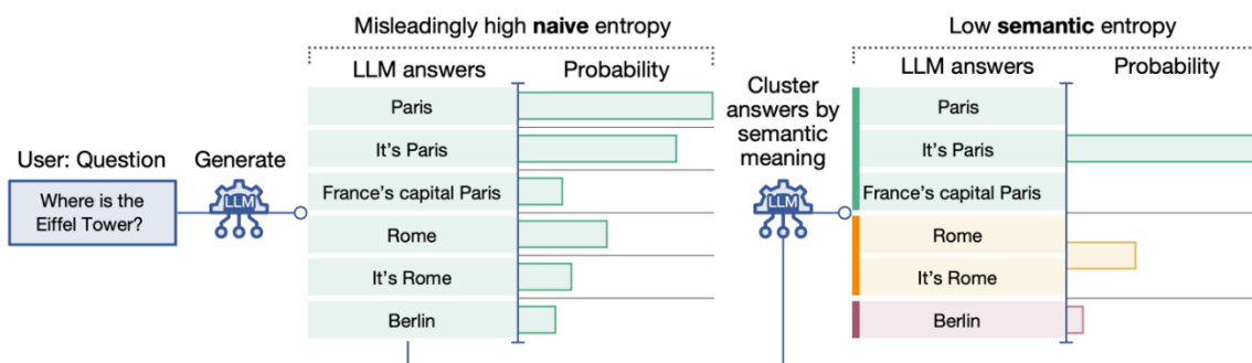
Fig. 4. Naive entropy-based uncertainty measures variation in the exact answers, classifying phrases such as "Paris," "It's Paris," and "France's capital Paris" as distinct entities. [50]
